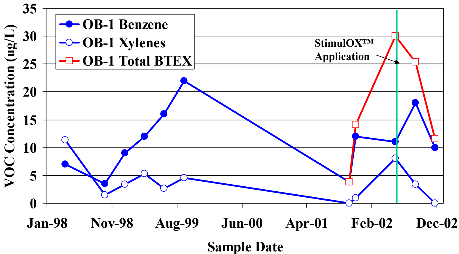
Figure 6. StimulOX™ Field Pilot Test Results for Side-Gradient Wells (outside of treatment area)
