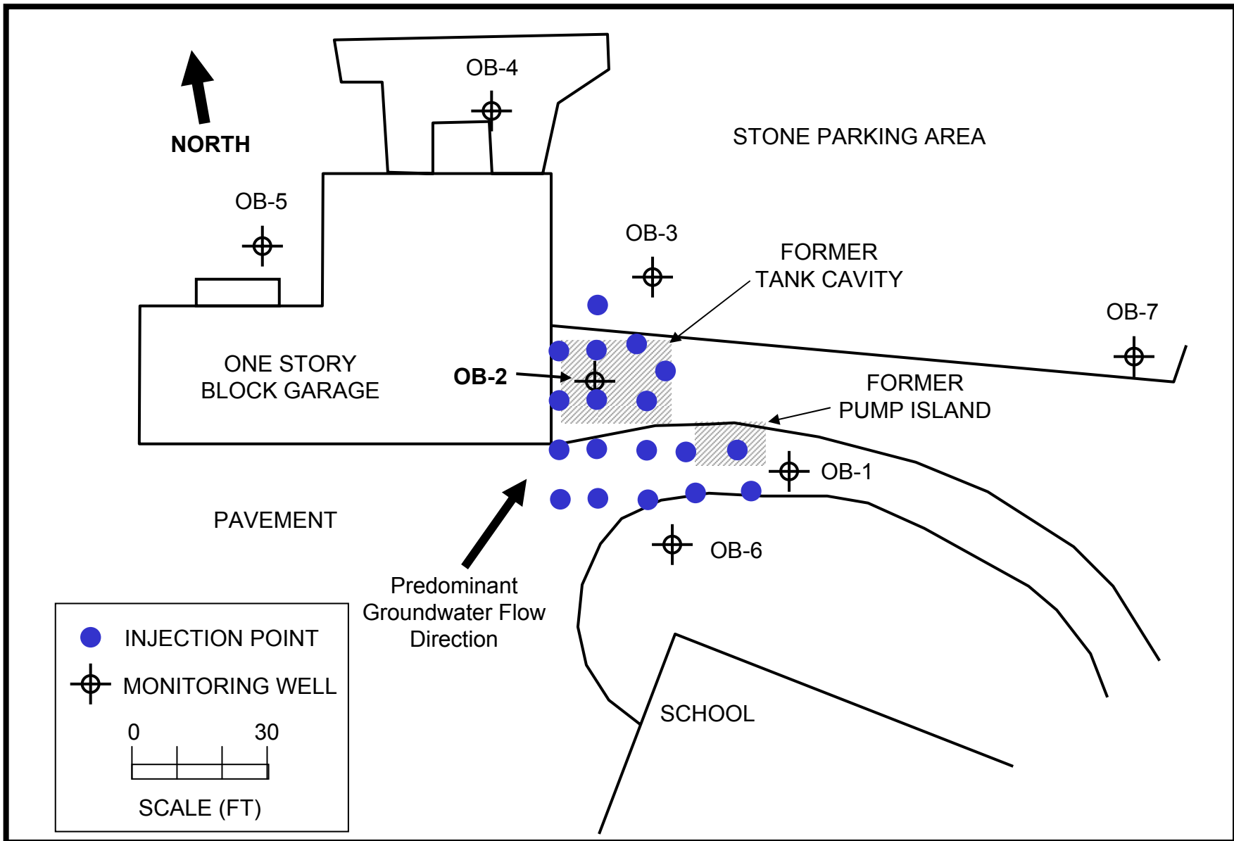
Figure 3. StimulOX™ Field Pilot Test Layout
