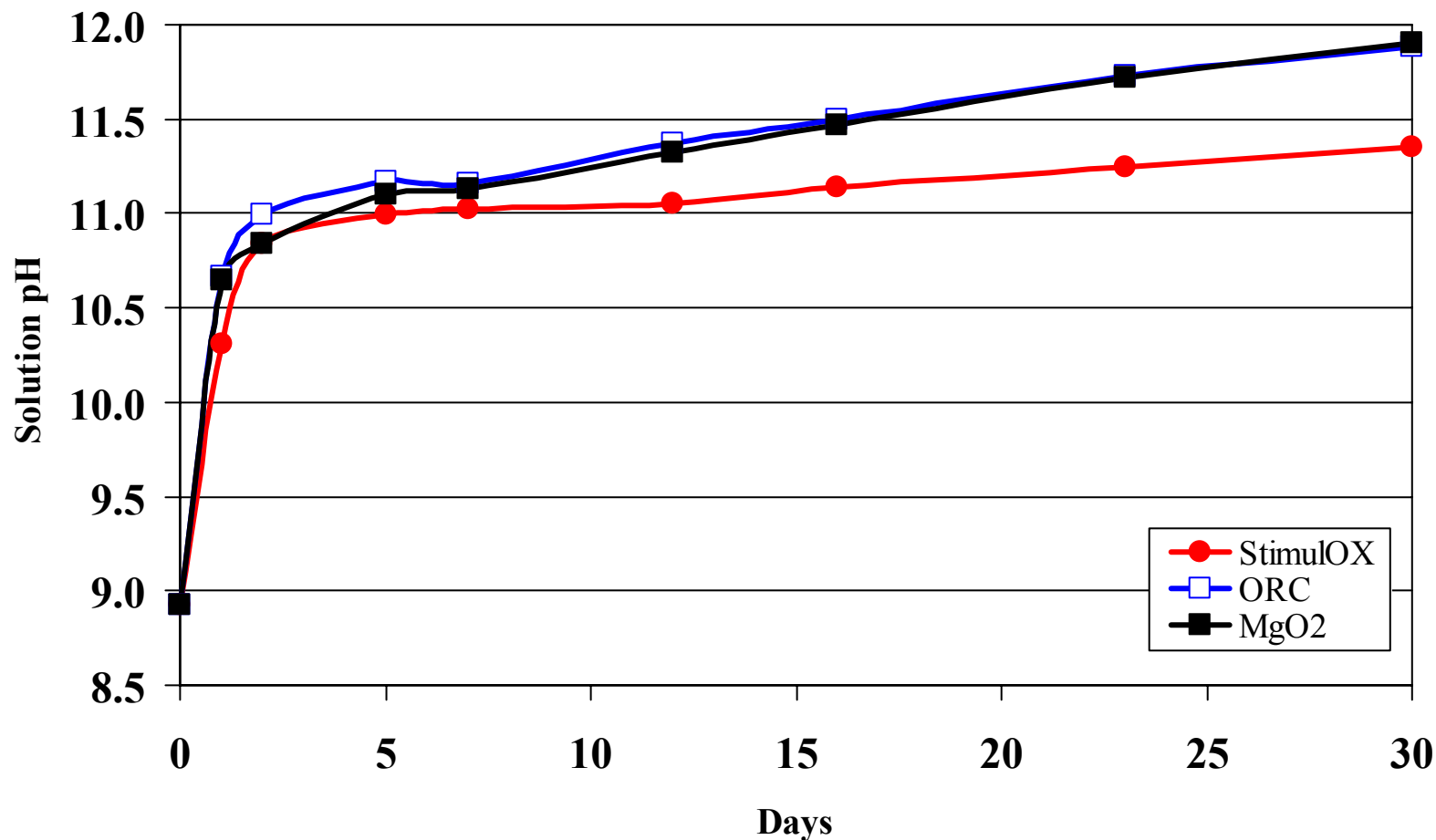
Figure 2. StimulOX™ pH Bench Test Results
