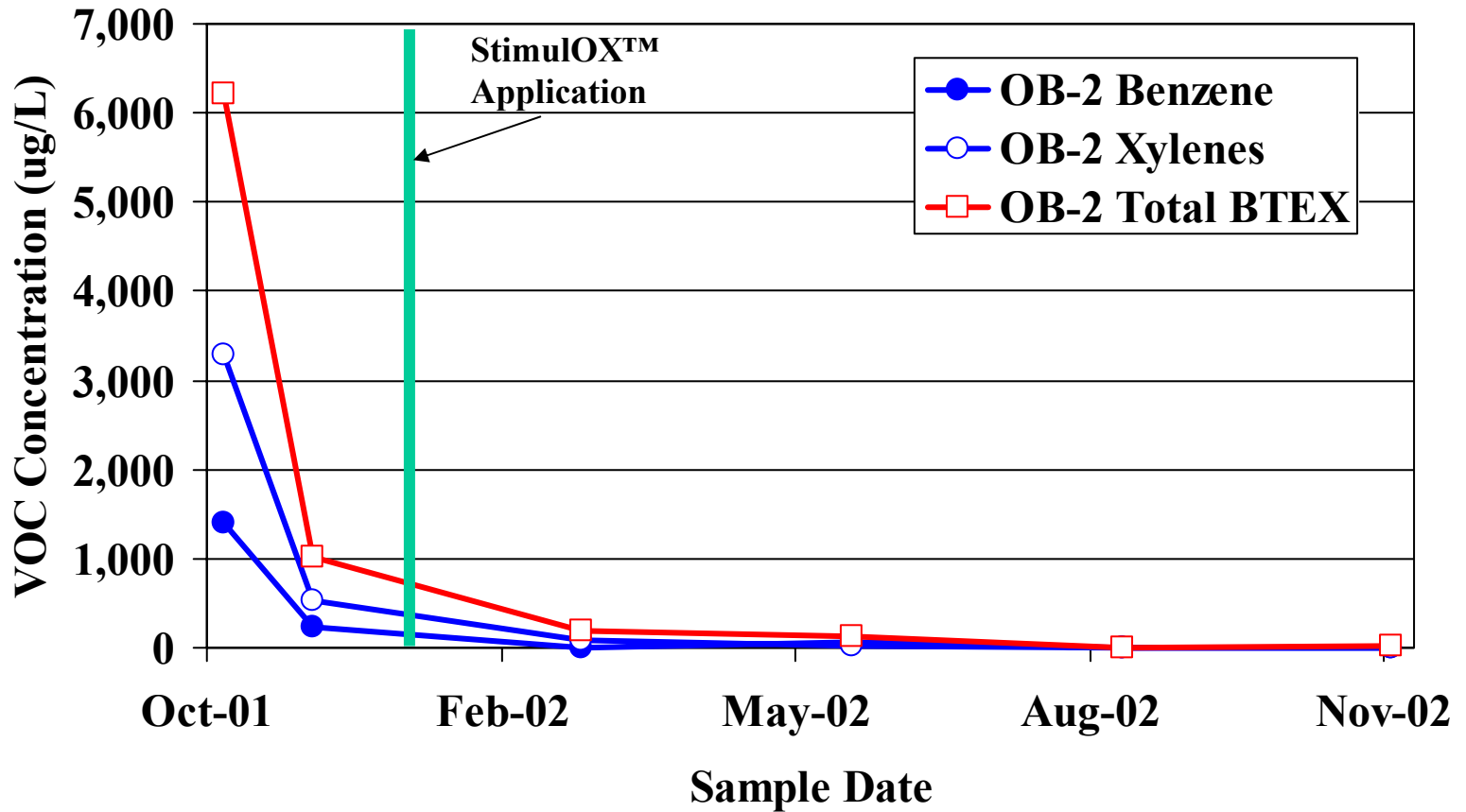
Figure 5. StimulOX™ Field Pilot Test Sampling Results for Source Area Well
