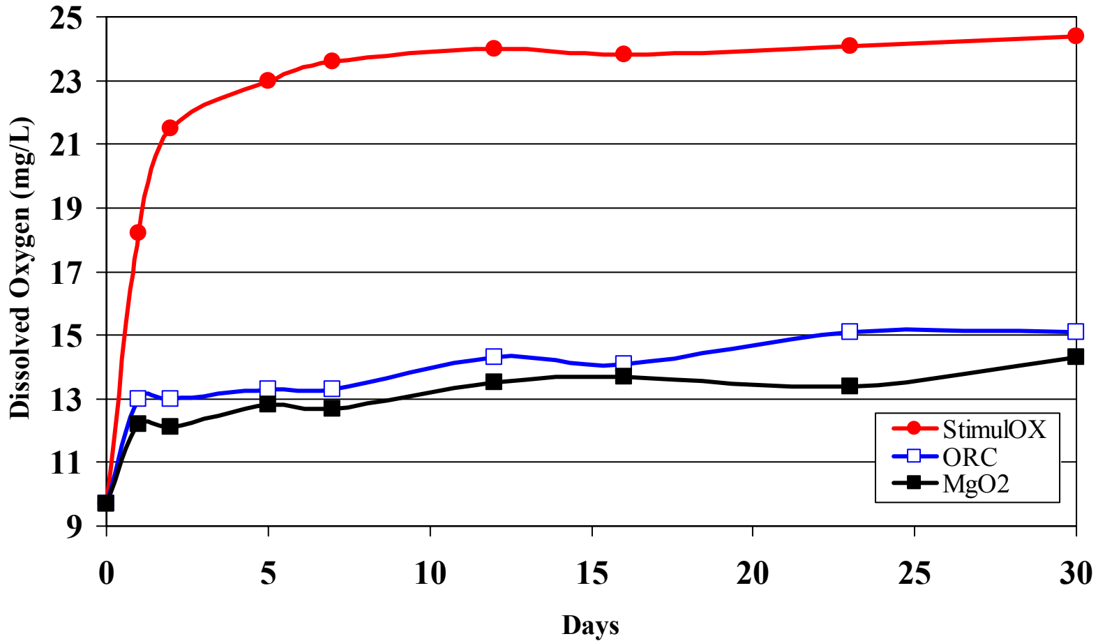
Figure 1. StimulOx Dissolved Oxygen Bench Test Results
